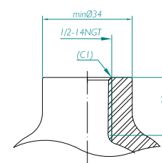
1/2-14NGT/CGA V-1
