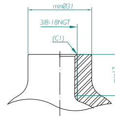
3/8-18NGT/CGA V-1
