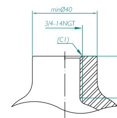
3/4-14NGT/CGA V-1
