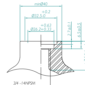
3/4-14NPSM/ASME B 1.20.1
